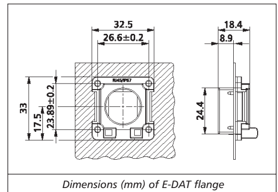
E-DAT size RJ45 to RJ45 coupler, 180° (optional)
