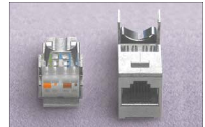
E-DAT size RJ45 jack to 8-pole IDC field cable termination (optional)
