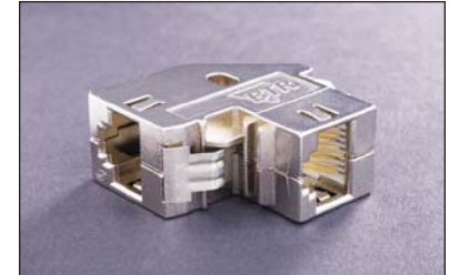
E-DAT size RJ45 to RJ45 coupler, 90° (optional)
