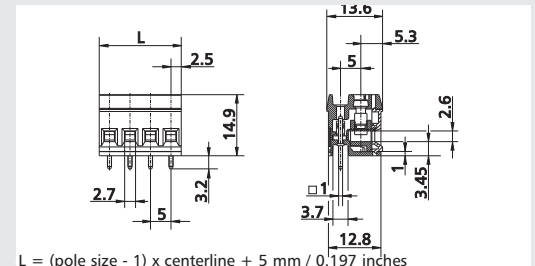
Dimensions in mm 1 mm = 0.0394 in.
