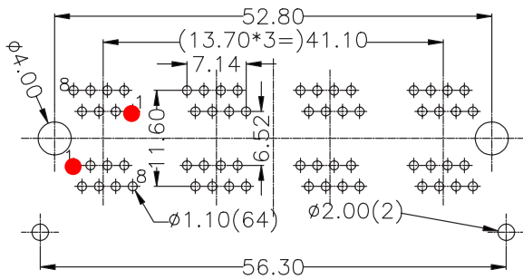
PC Board Layout - Component Side
