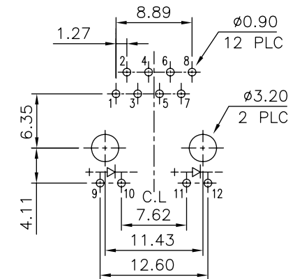
PCB Layout Ref.
