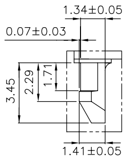
DETAIL X
