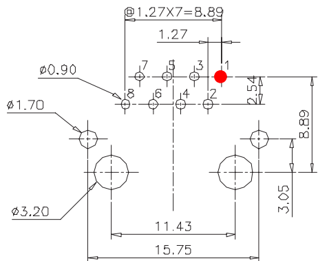
PC Board Layout - Component Side
