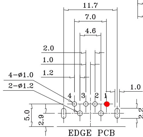
PC Board Layout - Bottom View ● = Pin 1
