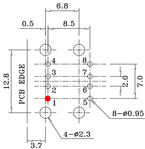
PC Board Layout - Bottom View
