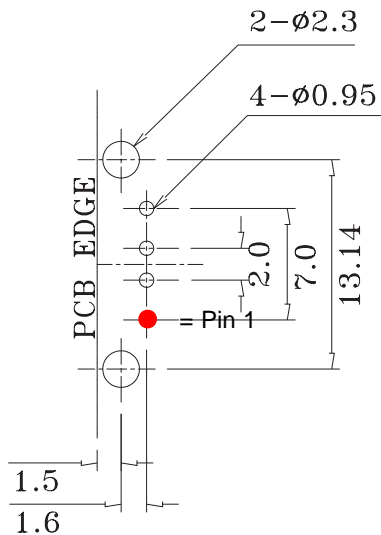
PC Board Layout - Component Side
