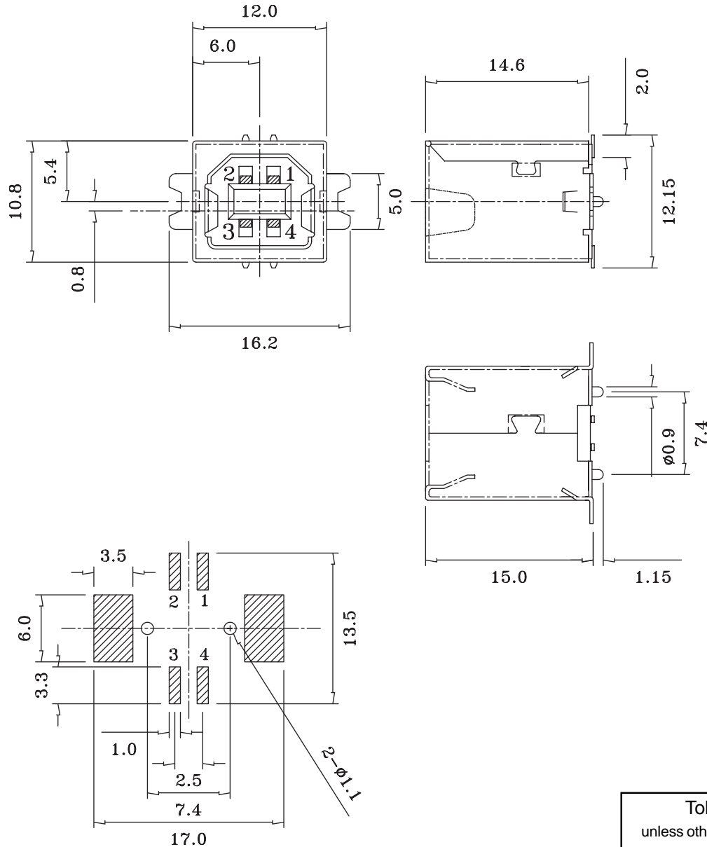
PC Board Layout - Component Side
