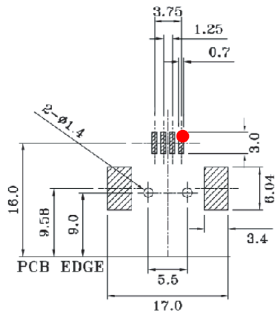
PC Board Layout - Component Side
