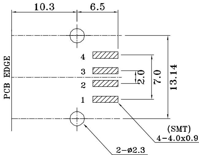
PC Board Layout - Bottom View
